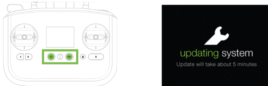
Figure 10.7.3: Controller Reset
