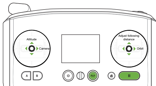
Figure 6.6.2.1: Follow Controls
