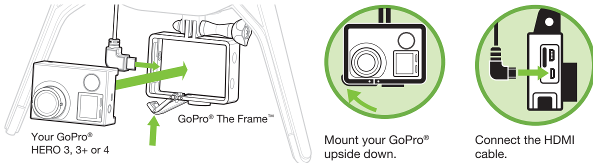
Figure 2.6.1.1: Attach Camera
