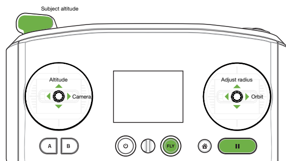
Figure 6.5.2.2: Orbit Controls
