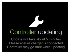
Figure 2.7.5.7: Controller - Updating
