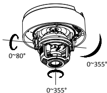
Figure 2-5 3-axis Adjustment
