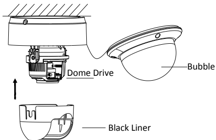
Figure 2-8 Install the Black Liner and Bubble
