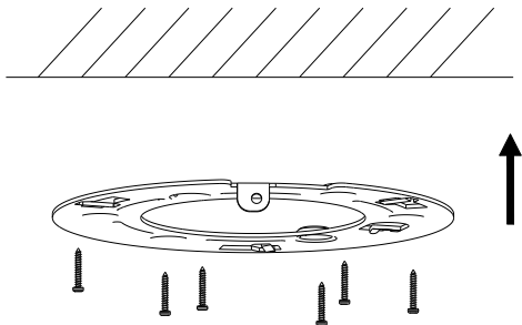
Figure 2-3 Install the Adapter Plate
