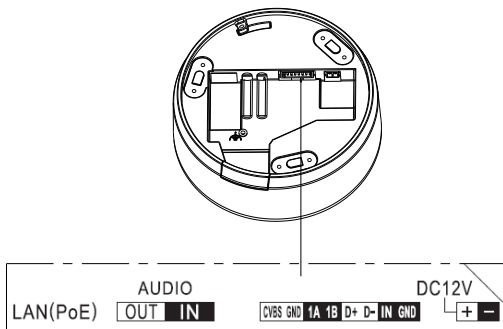
Figure 1-4 Overview (4)
