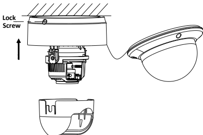
Figure 2-4 Install the Mounting Base
