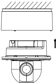
Figure 2-10 Install the Dome Drive
