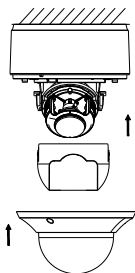
Figure 2-6 Install the Black Liner and Bubble
