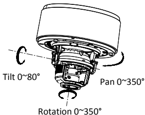
Figure 2-4 3-axis Adjustment
