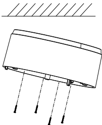
Figure 2-2 Install the Mounting Base
