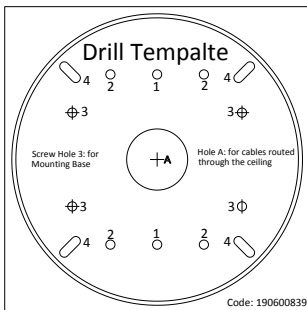
Figure 2-8 Drill Template
