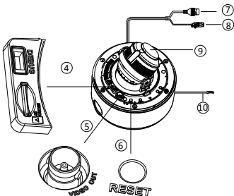
Figure 1-2 Overview (2) of Type II Dome Camera
