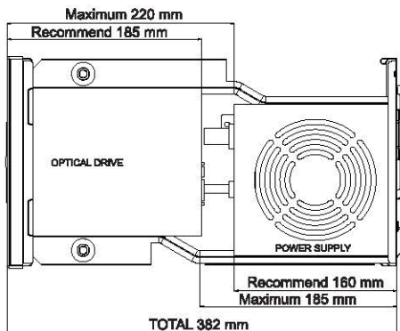
Power supply and optical drive figure
