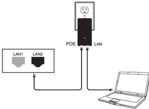
Connection diagram of POE with CPE
